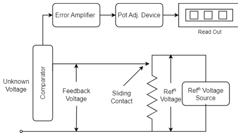
Fig: Servo Pot type DVM
