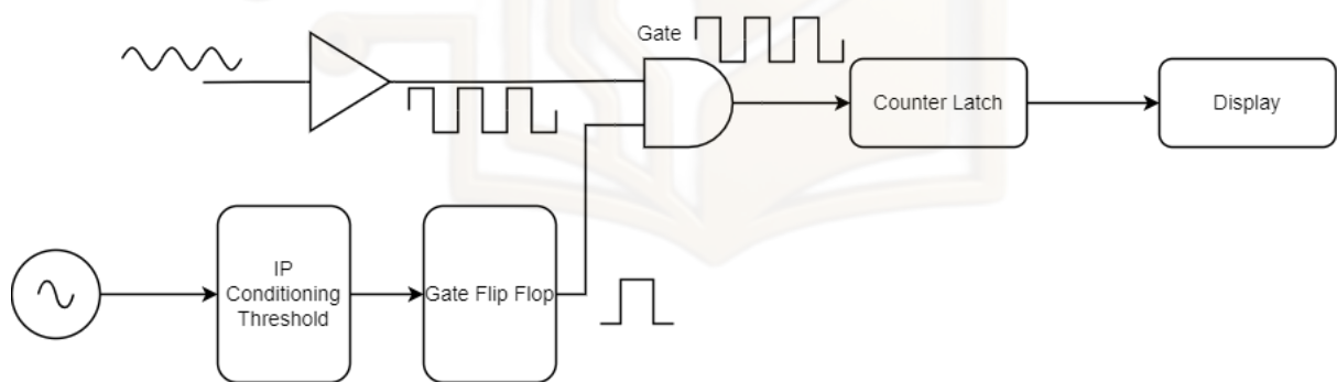
Fig: Frequency Counter
